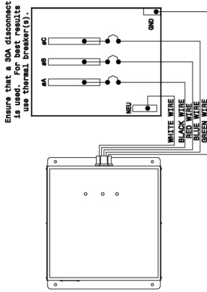
Figure 3 (Wye Models)
