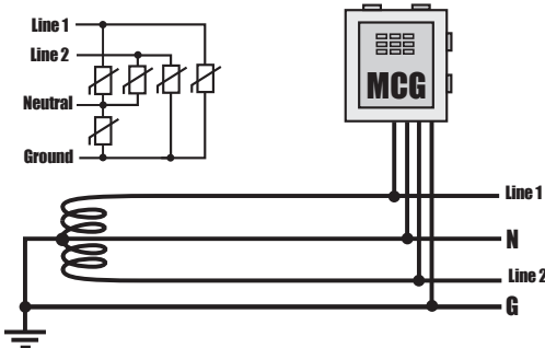
Single Phase, 3 Wire + Ground
